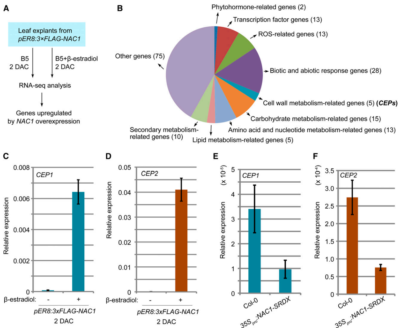
Figure 5. NAC1 promotes expression of CEP genes. A , RNA-seq analysis using 2-DAC leaf explants from pER8:3xFLAG-NAC1 . Leaf explants were cultured on B5 medium containing \beta -estradiol/DMSO or DMSO only (control). B , Analysis of upregulated genes in RNA-seq data as indicated in A . Also see Supplemental Table S2. C and D , qRT-PCR analysis of CEP1 ( C ) and CEP2 ( D ) transcript levels in leaf explants of pER8:3xFLAG-NAC1 cultured on medium without (–) or with (+) 10 \mu\text{M} \beta -estradiol at 2 DAC. E and F , qRT-PCR analysis of CEP1 ( E ) and CEP2 ( F ) transcript levels in leaf explants of 35S pro :NAC1-SRDX at 4 DAC. Bars in C to F show SD from three PCR experiments. Results were confirmed in two biological repeats. Data from one biological repeat are shown.
